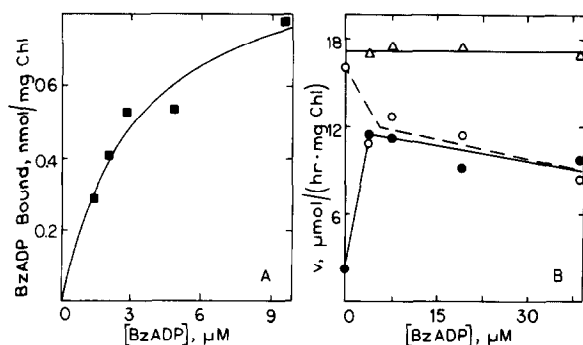
Fig.1. Non-covalent binding of BzADP to membrane-bound CF 1 . (A) Tight binding of Bz[ 3 H]ADP. Reaction conditions were as in section 2. Binding was quenched by the addition of 5 μM FCCP and 5 mM ADP. Tightly bound Bz[ 3 H]ADP was determined after release of the labeled analog by adding perchloric acid to the washed chloroplast thylakoids. The line was fit by non-linear regression [15]. (B) Protection, by BzADP, of P i -ATP exchange against inhibition due to ADP. BzADP at the indicated concentrations was added alone (○) or together with 5 μM ADP (●) in the dark 5 s after the activation step, and ATP + 32 P i (5 mM each) were added after an additional 60 s after the activation step.
